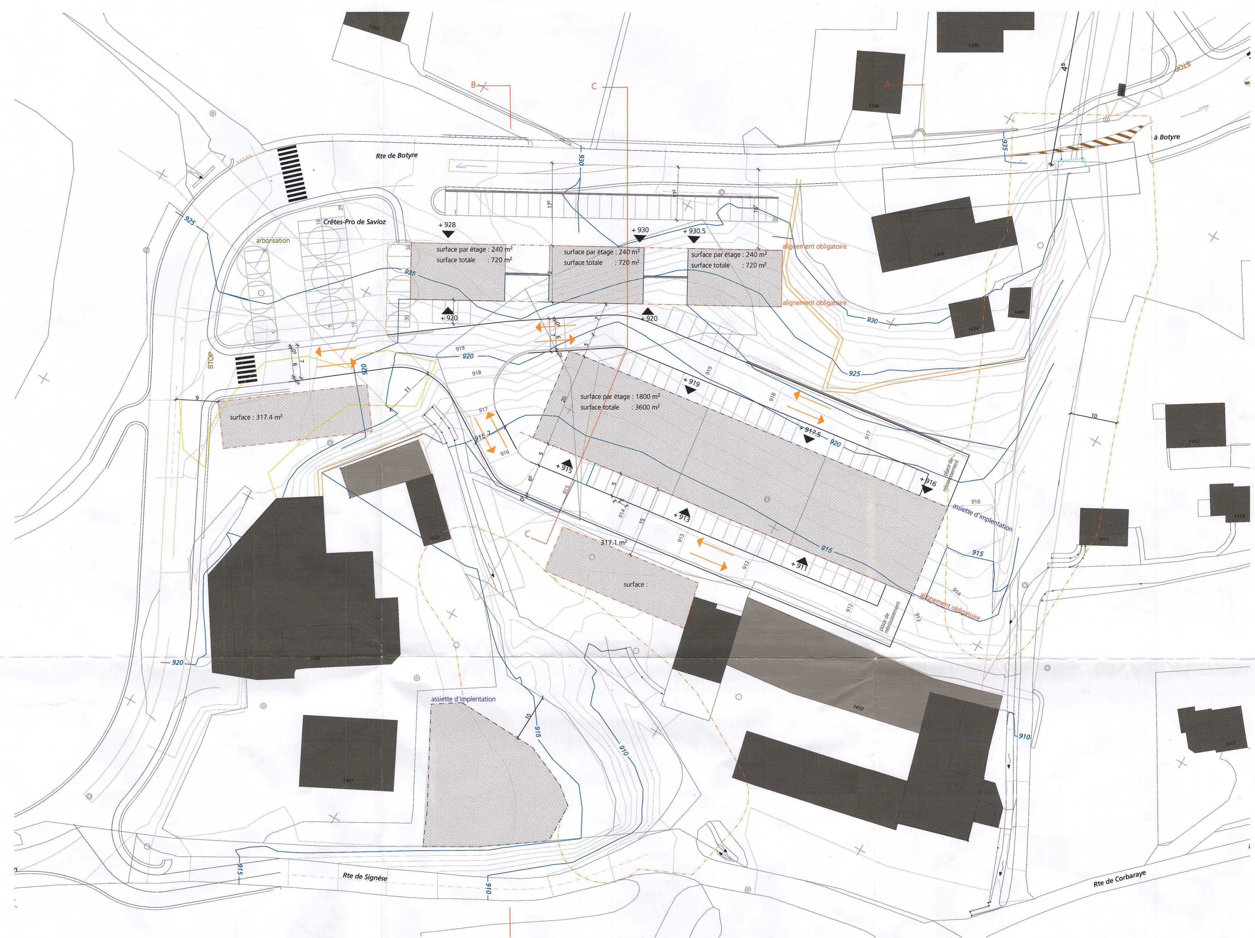
Plan situation 1/500
